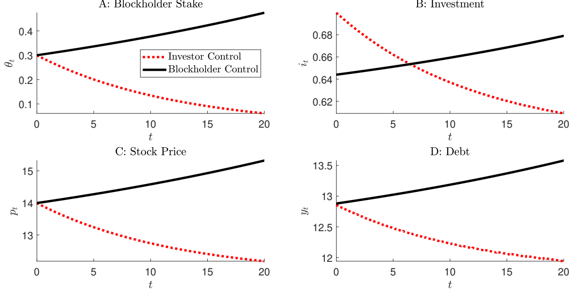
Figure 2: Model Dynamics and Control. We numerically calculate the equilibrium both under blockholder control (baseline; solid black line) and investor control (dotted red line). The parameters are \alpha = \kappa = 1 , \rho + \delta = 0.2 , r + \delta = 0.1 , \lambda = 0.25 , \mu = 0.05 , and \pi = 0.4 , as well as \tilde{\theta} = 0.99 and \pi^I = 1 . We set \theta_0 = 0.3 .
