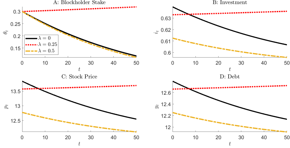
Figure 1: Agency Conflicts and Model Dynamics. We numerically calculate the equilibrium both under varying levels of agency conflicts \lambda . The parameters are \alpha = \kappa = 1 , \rho + \delta = 0.2 , r + \delta = 0.1 , \lambda = 0.25 , \mu = 0.05 , and \pi = 0.5 , as well as \tilde{\theta} = 0.99 and \pi^I = 1 . We set \theta_0 = 0.3 .
