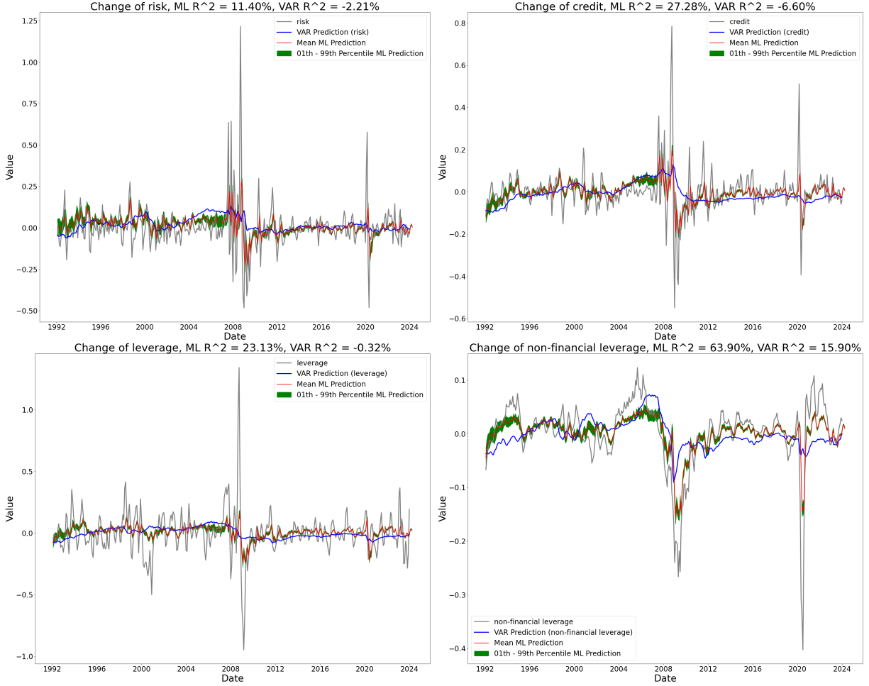
Figure 13: Predicting macroeconomic variables using neural network and VAR
