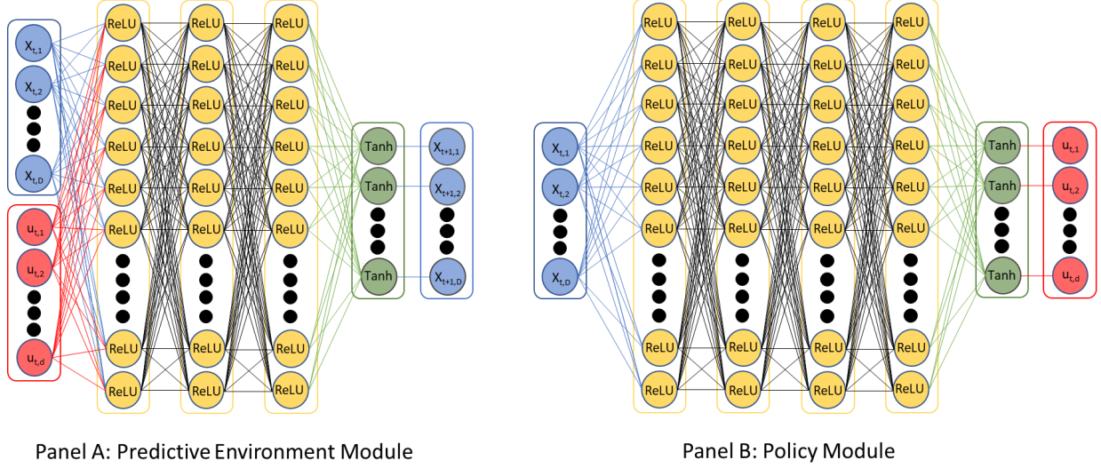
Figure 2: AlphaManager (AM) Architecture
