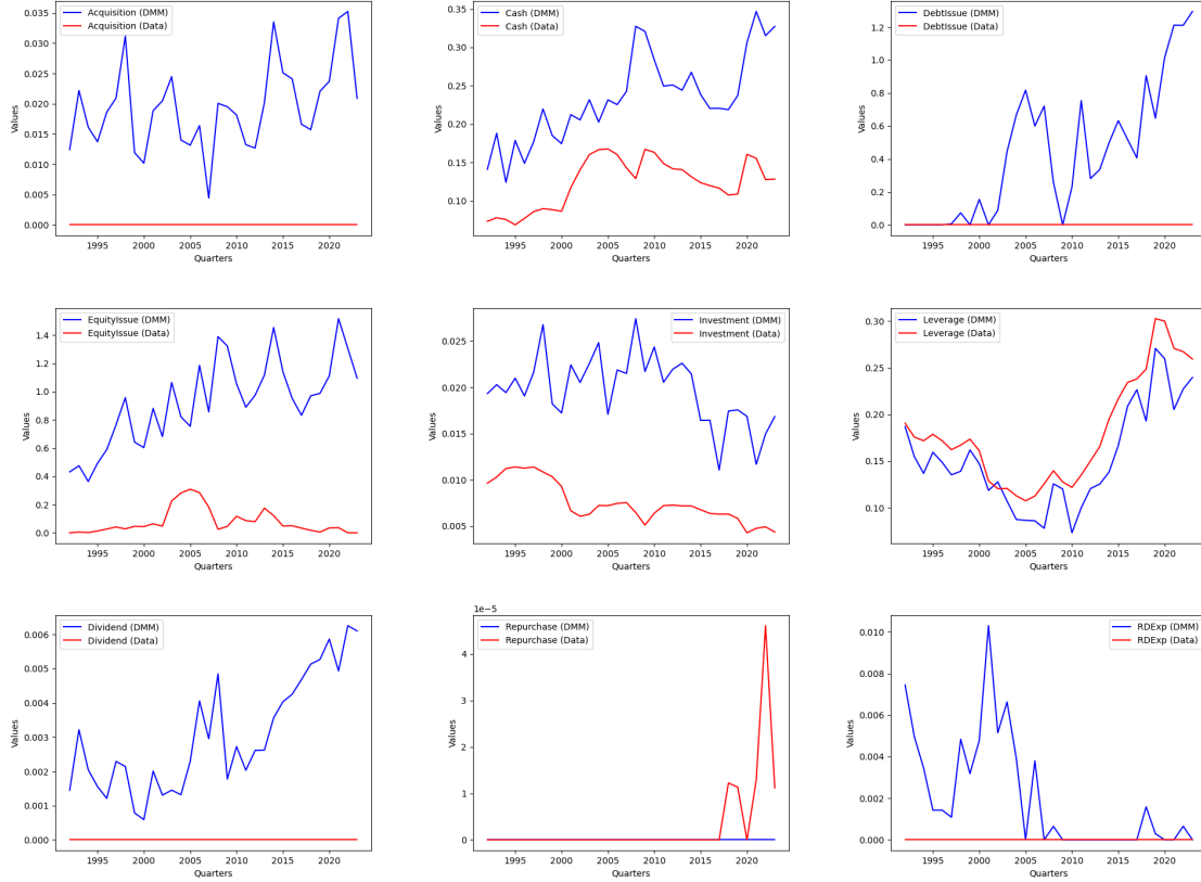
Figure 9: Empirical and Optimal Decisions under 1-QTR Enterprise Value Growth
