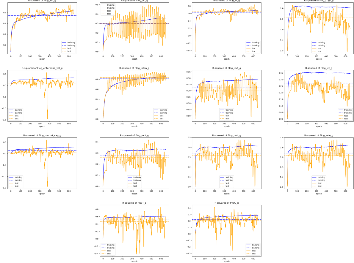
Figure 3: PEM: In-Sample and Out-of-Sample Pseudo R^2 for System States
