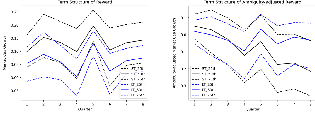
Figure 7: Term Structure of Reward and Ambiguity-adjusted Reward
