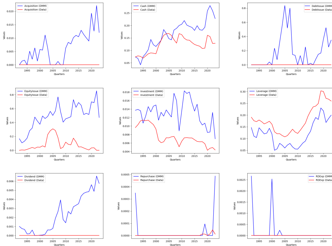
Figure 10: Empirical and Optimal Decisions under 8-QTR Market Cap Growth
