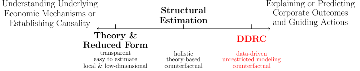
Figure 1: Contrasting Corporate Finance Research Approaches
