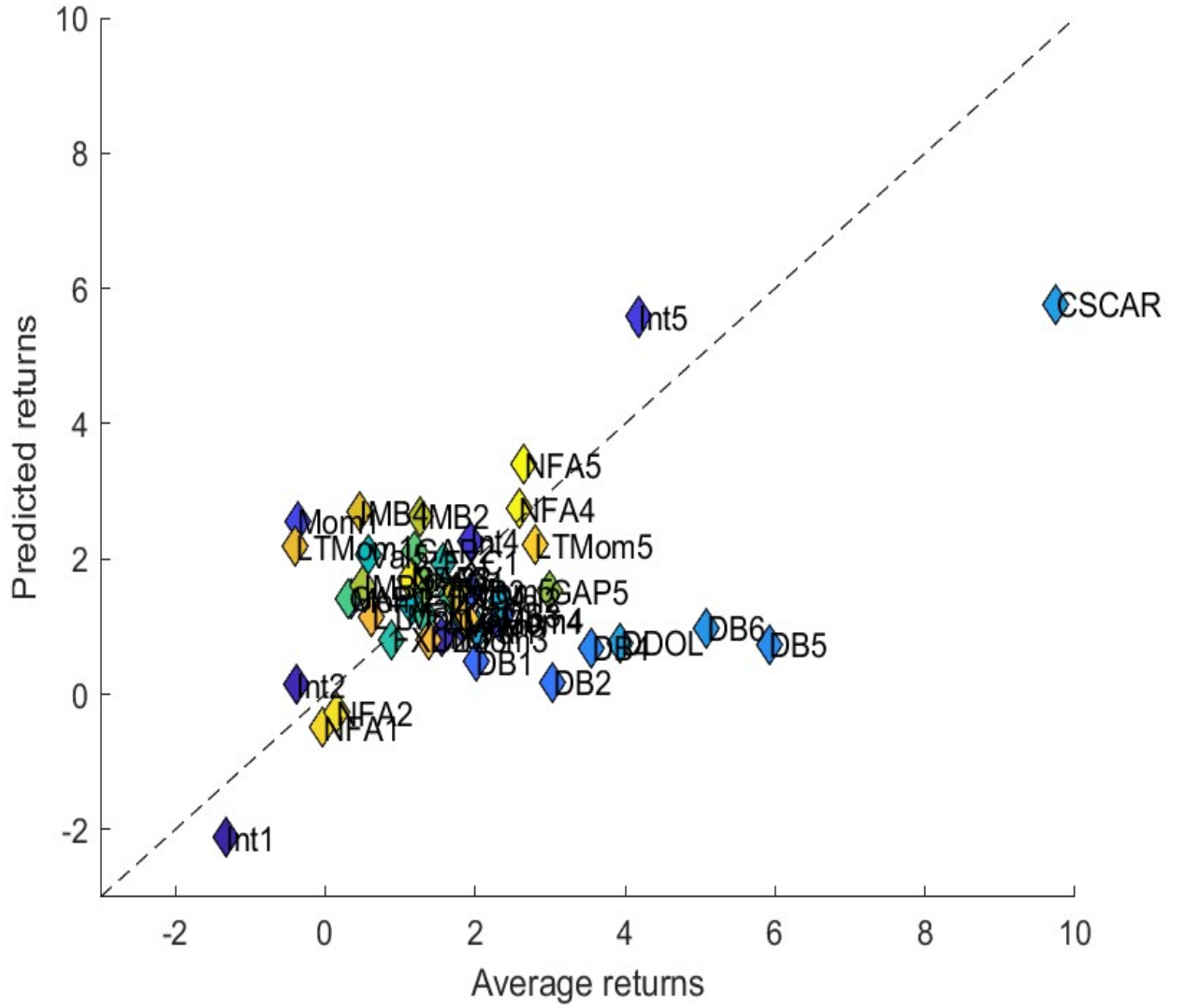
Figure 1: Scatter plot of average vs model implied returns. The model implied returns are based on the GMM estimates (Table 3) of the unconditional DOL-CAR model using 36 test assets constructed from our set of 29 developed and emerging currencies from December 1983 to March 2024.
