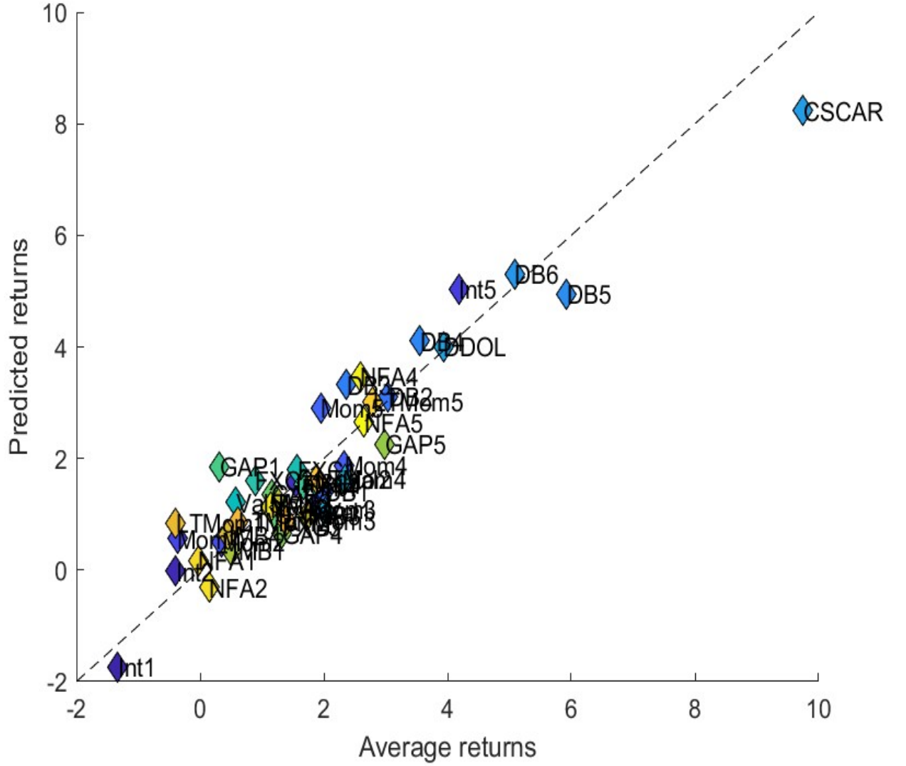
Figure 3: Scatter plot of average vs model implied returns. The model implied returns are based on the GMM estimates (Table 3) of the unconditional DOL-CAR model with \delta = 1 using 36 test assets constructed from our set of 29 developed and emerging currencies from December 1983 to March 2024.
