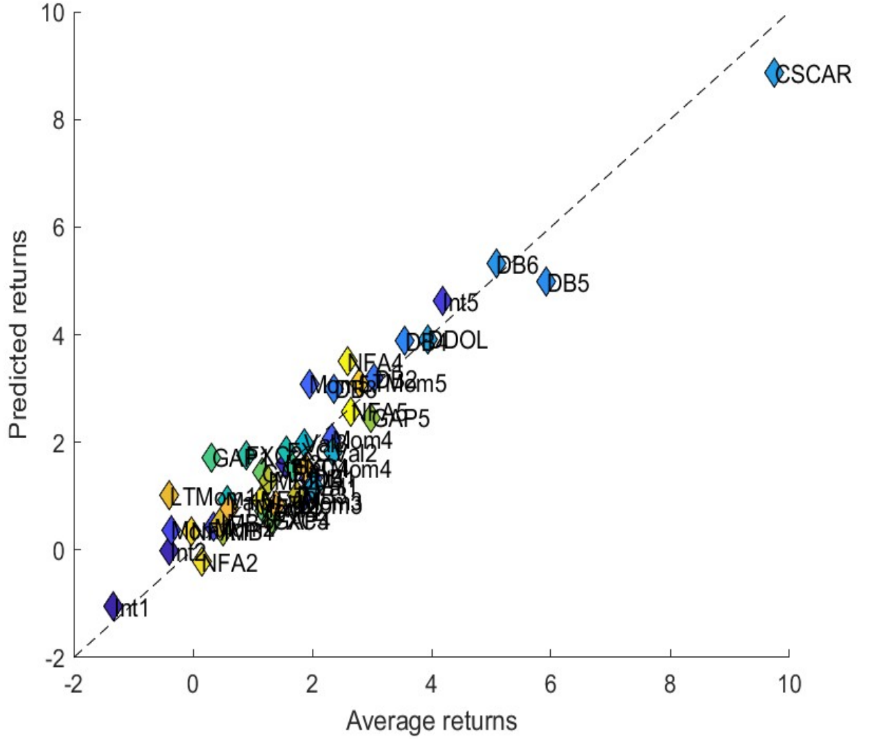
Figure 2: Scatter plot of average vs model implied returns. The model implied returns are based on the GMM estimates (Table 3) of the conditional DOL-CAR model with free \delta using 36 test assets constructed from our set of 29 developed and emerging currencies from December 1983 to March 2024.
