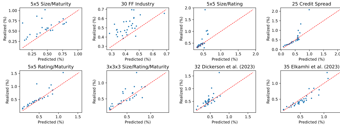
Figure 6: Realized vs. Predicted Returns at the Portfolio Level with Rolling-Window Betas
