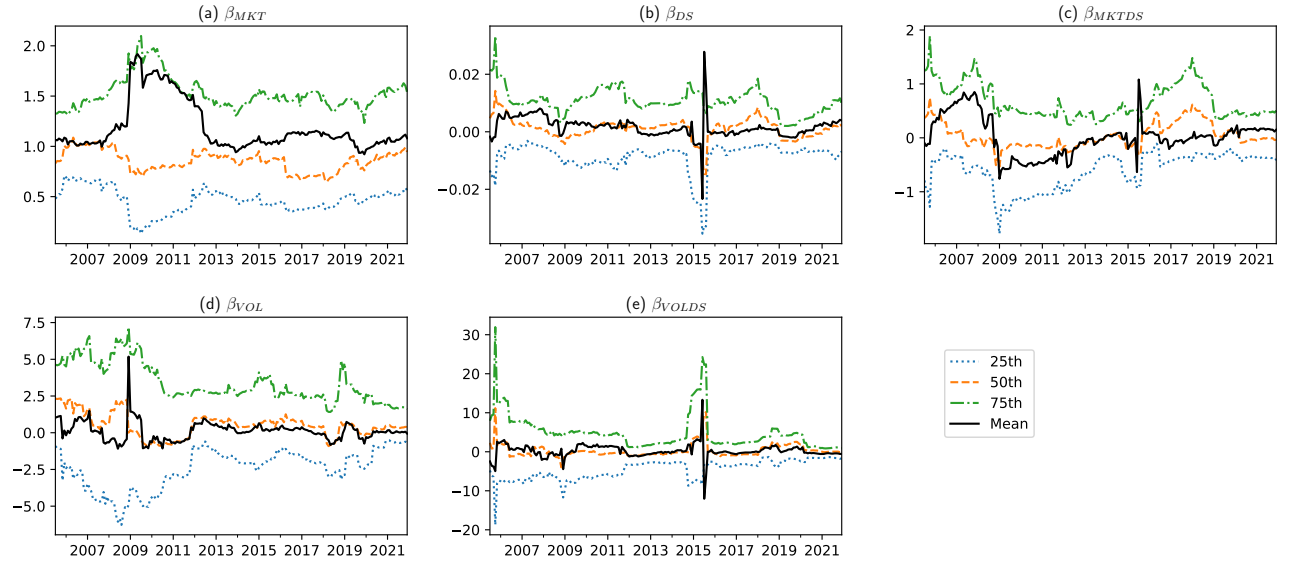
Figure 2: Time-Series Distribution of Estimated GDA5 Factor Betas
