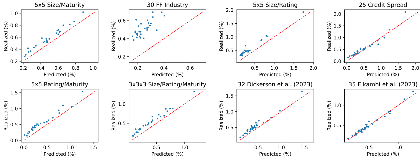
Figure 5: Realized vs. Predicted Returns at the Portfolio Level with Unconditional Betas
