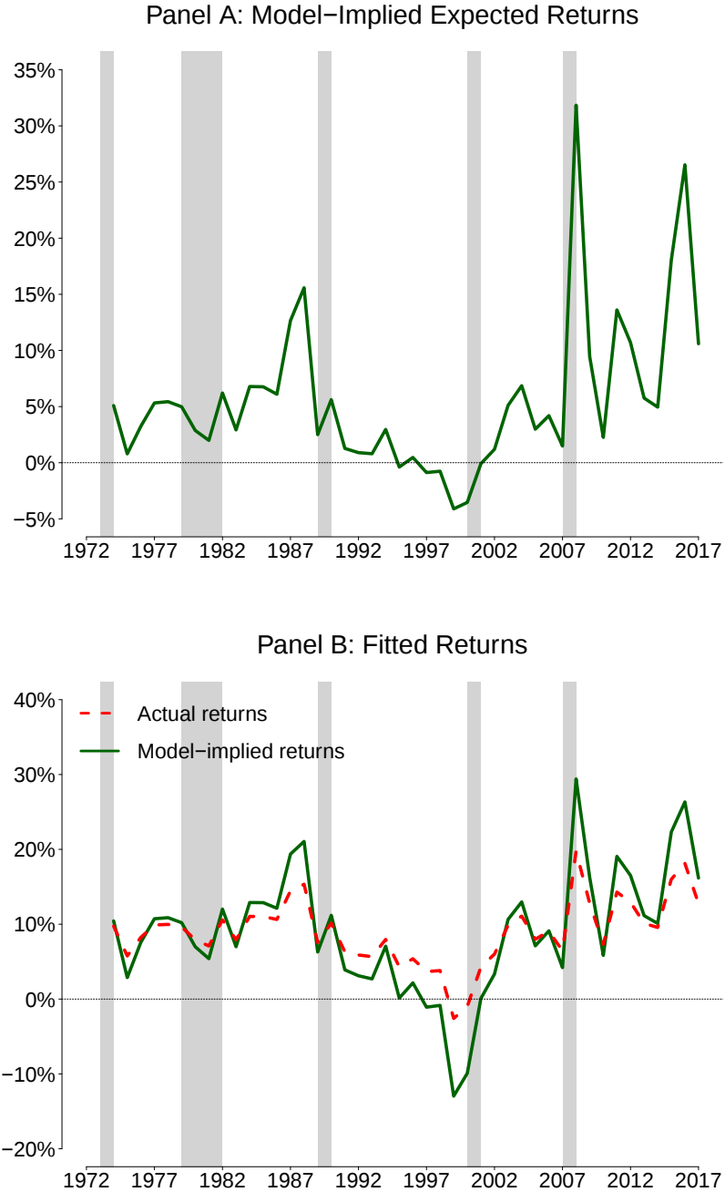
Fig. 4: Properties of model-implied expected returns
