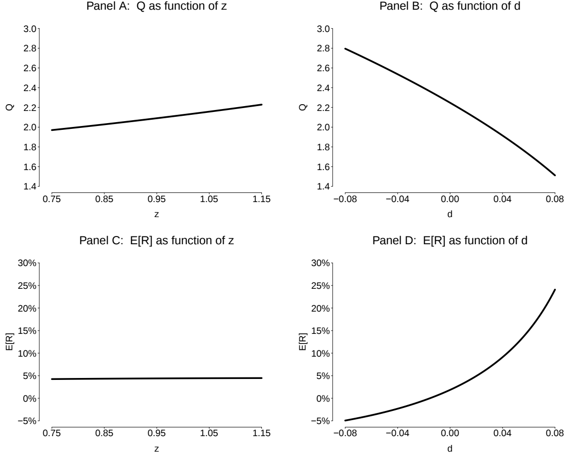
Fig. 2: Model-implied Q and expected firm return as functions of the state variables
