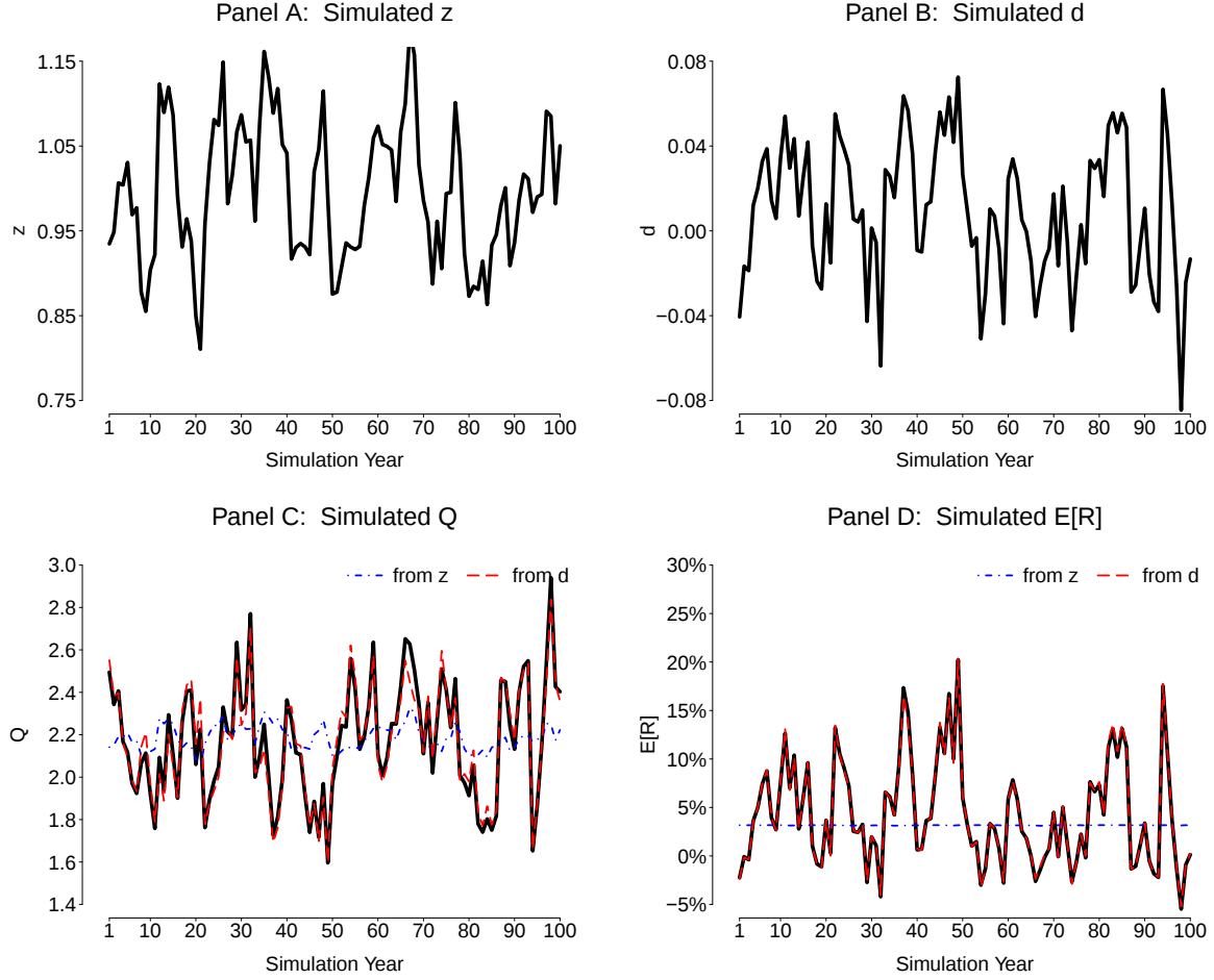
Fig. 3: Simulated paths: model with unlevered firm
