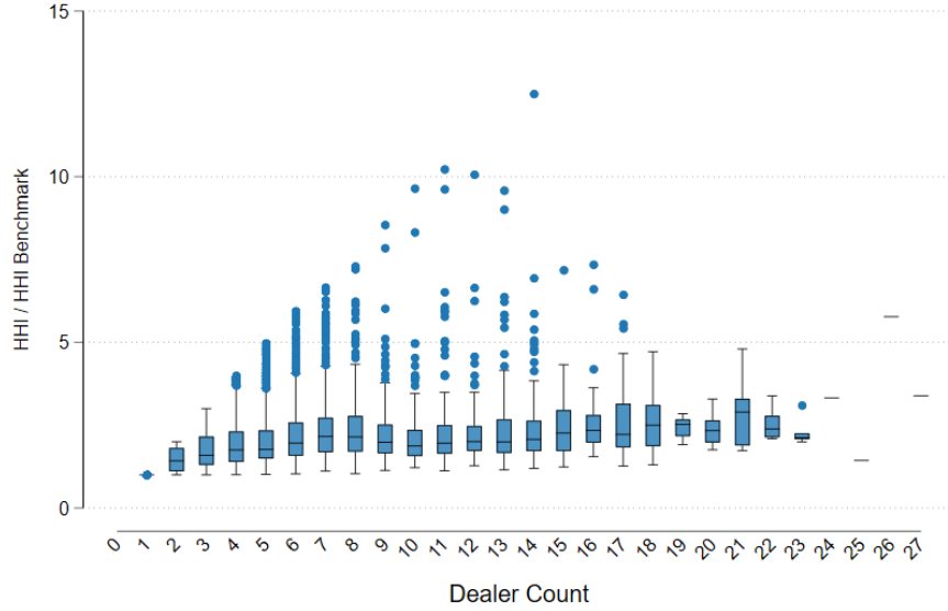
(b) \frac{HHI_i}{EqualDistribHHI} by DealerCount_i .
