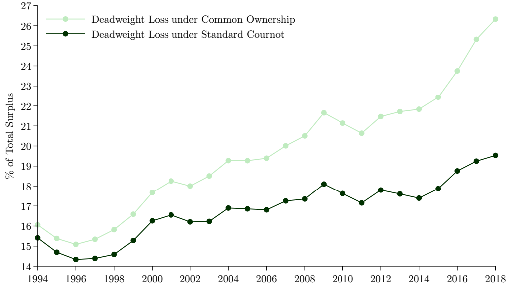
FIGURE NOTES: The figure plots the estimated deadweight loss (DWL), net of fixed costs and minimum profits, of oligopoly and of oligopoly and common ownership between 1994 and 2018. The dark green line is the DWL of oligopoly as measured by the % difference in total surplus between the Cournot equilibrium and the Perfect Competition scenario. The light green line is the DWL of oligopoly and common ownership as measured by the % difference between the Cournot Common Ownership equilibrium and the Perfect Competition scenario.
